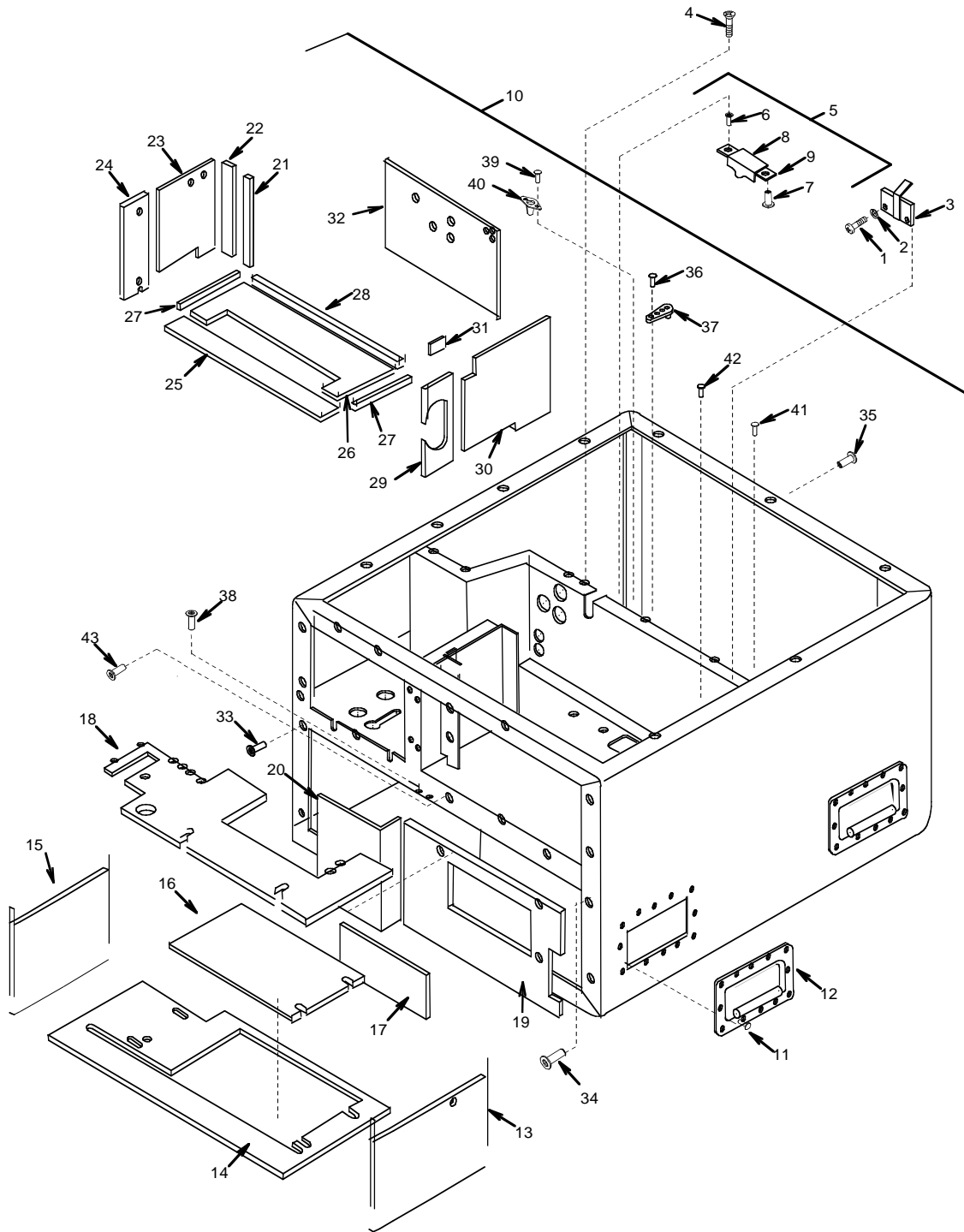
Figure 20. Housing
