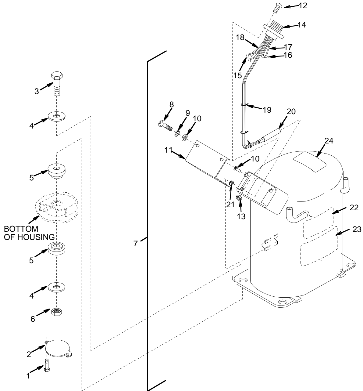
Figure 19. Compressor
