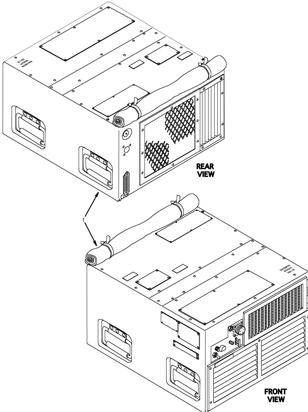
Figure 1. Air Conditioner
