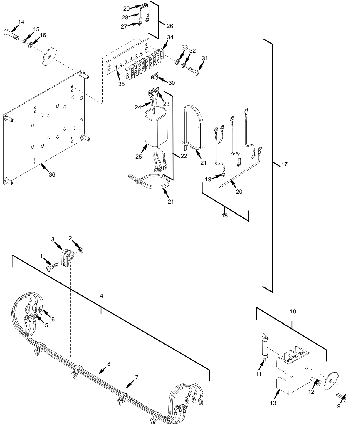
Figure 12. Power Factor Improvement Components
