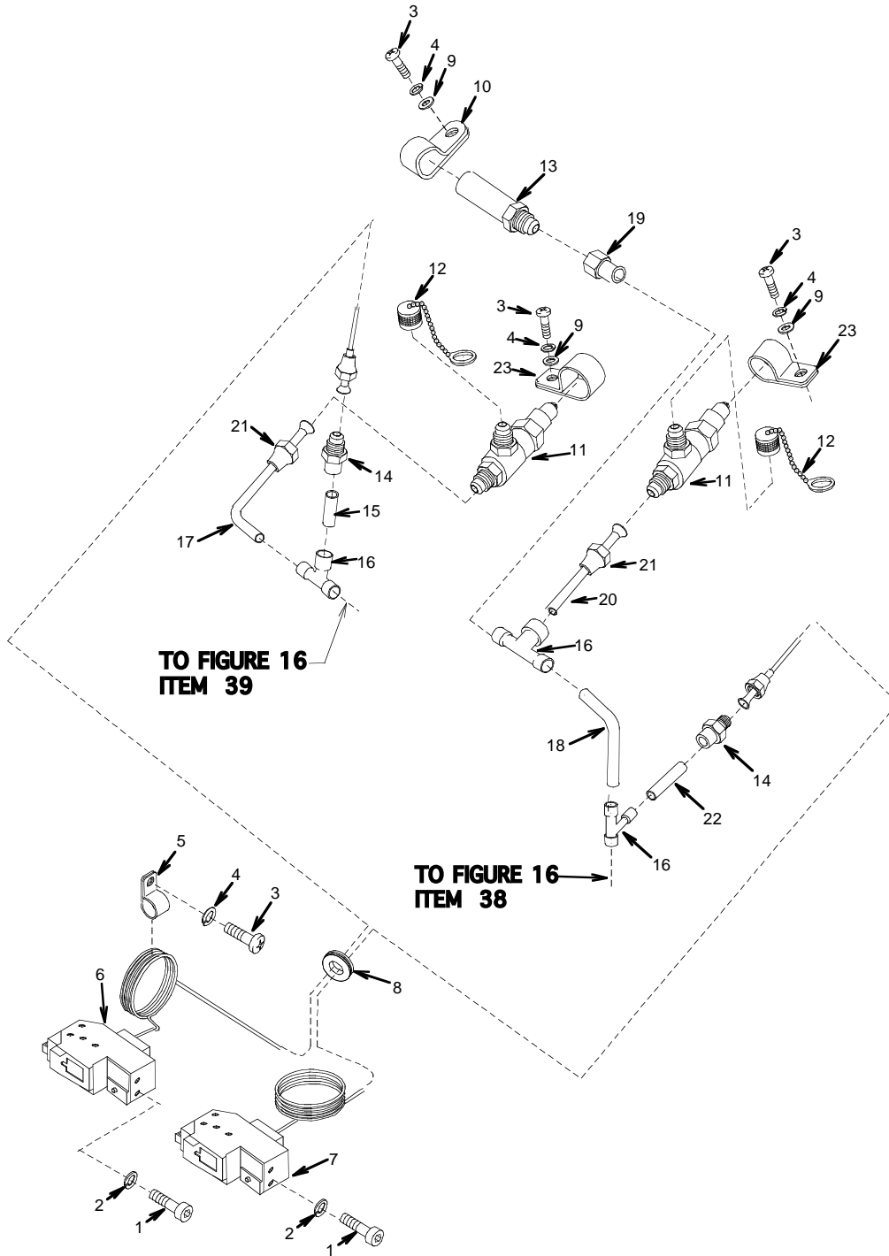
Figure 17. Pressure Switches, Charging Valves, and Relief Valve
