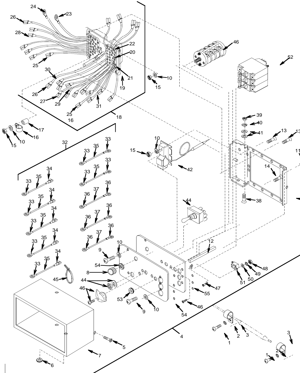
Figure 8. Control Module
