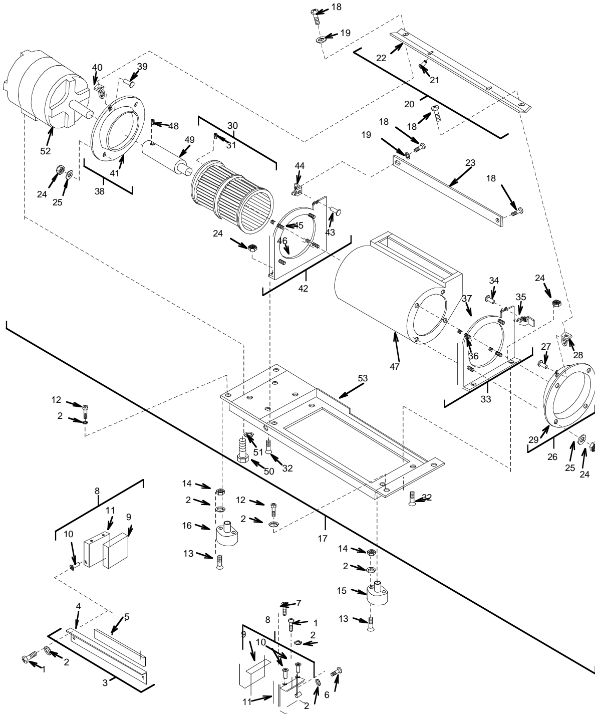
Figure 13. Evaporator Fan Assembly
